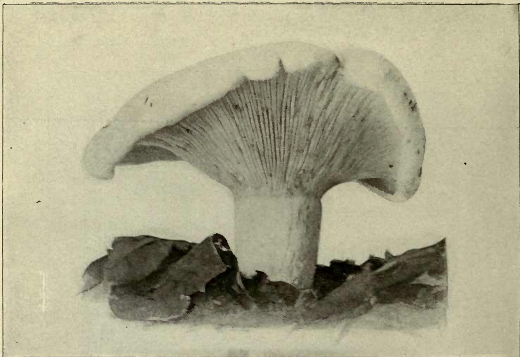
PEPPERY LACTARIUS
