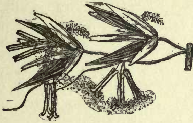
Grass spikelet
