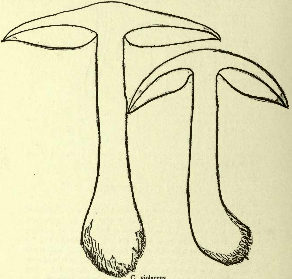
C. violaceus
