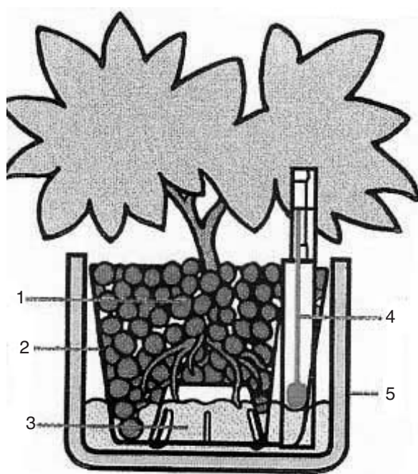
Figure 11.8 Hydroculture system for growing plants in a small pot (1: clay pellets, 2: culture pot insert, 3: nutrient solution, 4: water level indicator, 5: outer container). A constant level of nutrient solution is maintained in the bottom of the outer container, with nutrient solution added through the water level indicator opening. Source: Angus, J., 1995–96, The Growing Edge 7(2):48–55.
