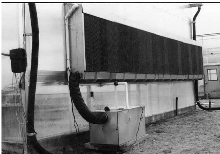
Figure 12.7 Cooling pad placed at one end of the greenhouse. Air is pulled through the cooling pad by exhaust fans placed at the opposite end of the greenhouse — see Figure 12.6. Water is passed over the cooling pad. As shown here, the large box set on the ground contains water, which is pumped to the top of the cooling pad and allowed to flow down the pad and then is collected and flows back into the water storage box.
