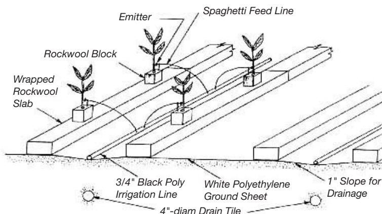
Figure 9.10 Visual sketch of a rockwool slab with a plant-containing cube placed on the slab and a drip line in place. Source: Resh, H.M., 1995, Hydroponic Food Production, 5th ed., Woodbridge Press Publishing, Santa Barbara, CA.
