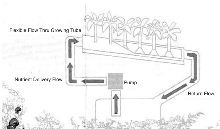
Figure 9.2 A typical arrangement for a closed NFT system in which nutrient solution is pumped from a storage tank into the sloping NFT trough and then by gravity the nutrient solution flows back into the storage tank.
