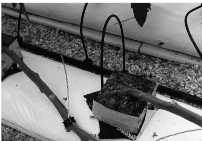
Figure 9.6 Drip irrigation line (black tubing) positioned on a rockwool block set on a perlite-containing bag.
