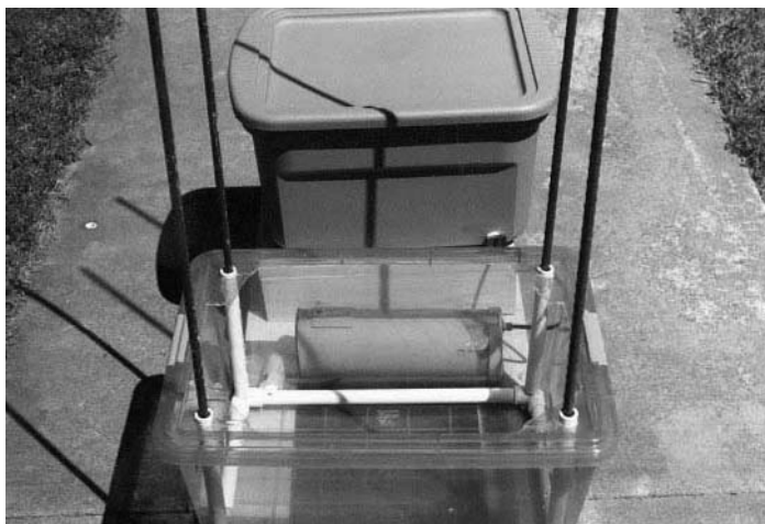
Figure 11.9–1 GroSystem GroBox hydroponic system. (The PVC piping in the rooting box is used to support the four corner plant stakes, the blue PVC pipe houses a float value used to maintain a constant level of nutrient solution in the base of the rooting box, and the green plastic box contains the nutrient solution. A tube is inserted in the base of nutrient solution box to deliver nutrient solution to the float value.)
