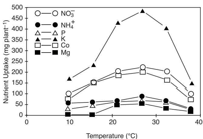
Figure 11.21-1 Influence of root zone temperature on major nutrient element uptake. Source: Tindall, J.A., Mills, H.A., and Radcliffe, D.E., 1990. The effect of root zone temperature on nutrient solution uptake of tomato, J. Plant Nutr. 13:939–956.
