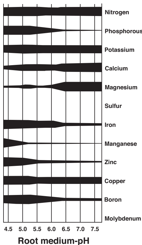
Figure 7.2 Effect of root medium pH on the availability of the essential elements affecting root absorption in an organic soilless mix. (Source: Agroand Fisher (2003))
