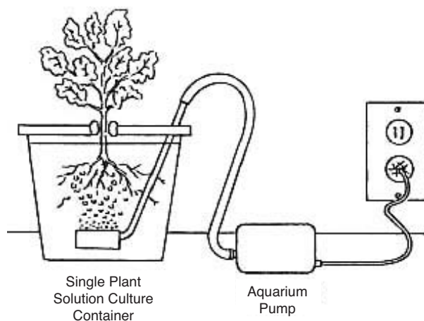
Figure 9.1 Standing aerated nutrient solution hydroponic growing system with the aquarium air pump attached to a line to a dispenser in the bottom of the growing vessel so that air can be bubbled into the nutrient solution.
