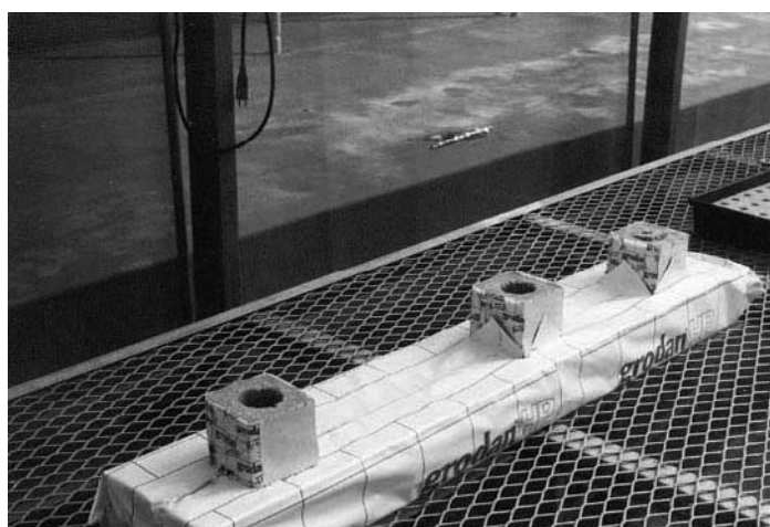
Figure 9.9–2 A typical rockwool slab with rockwool cubes spaced as would be appropriate for growing tomato.
