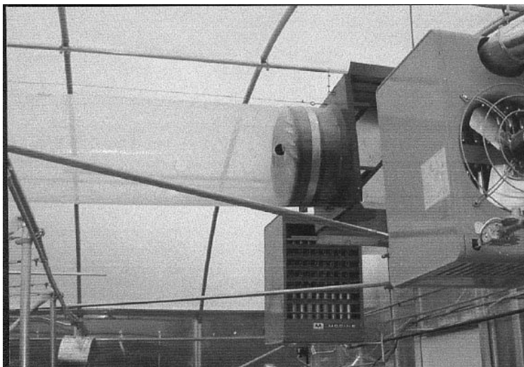
Figure 12.8 Natural gas- or propane-fired jet fan heater placed in the gable at the ventilation fan end of the greenhouse (common method of heating and dispersing hot air into a greenhouse).
