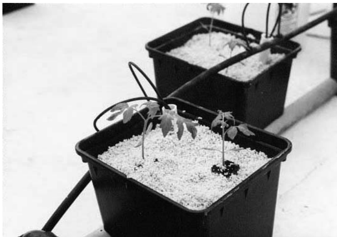
Figure 9.7 Drip irrigation line (large black tubing is the delivery line, the smaller tubing the drip tube) for delivering nutrient solution to perlite-filled BATO buckets.
