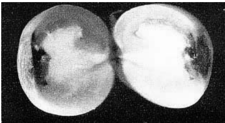
Figure 11.25 Symptoms of blossom-end rot (BER) on tomato fruit. Normally, the symptom — browning (decay) of the blossom end of the fruit — occurs early in fruit development. Such fruit should be removed when first observed. BER fruit will early turn red.
