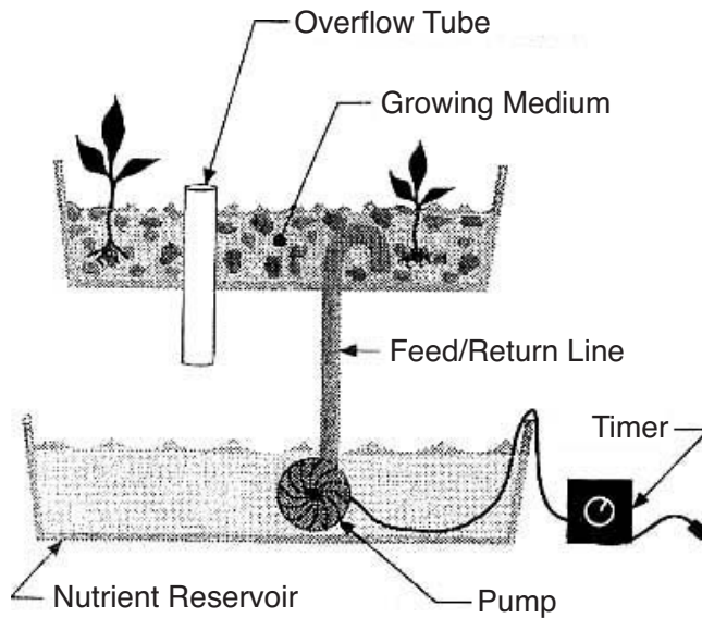
Figure 9.5 Flood-and-drain (ebb-and-flow) hydroponic growing system. Periodically, nutrient solution is pumped from the nutrient reservoir into the growing medium, flooding the medium with nutrient solution which is then allowed to drain back into the nutrient reservoir. (Source: Van Patten, G.P., 1992, The Growing Edge 3(3): 24–33, 48–51).
