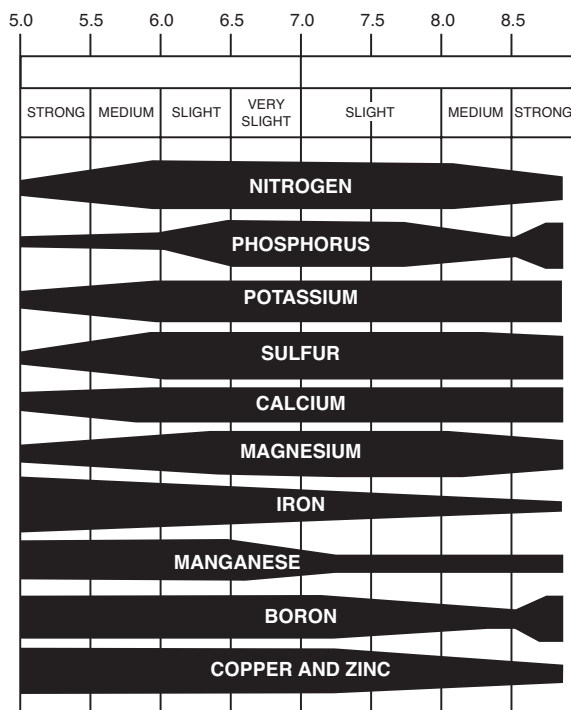
Figure 7.1 Effect of pH on the availability of the essential elements affecting root absorption in a mineral soil.
