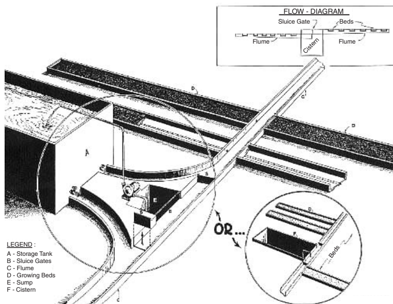
Figure 11.2 Basic drawing of an ebb-and-flow (flood-and-drain) hydroponic growing system in common use in the past for growing a wide range of crops. Stored in the base or sump under the growing bed, a nutrient solution is pumped into the growing bed above (usually containing gravel of similar inert coarse material), flooding the bed, and then after a short time, the nutrient solution flows by gravity back into the sump. In this drawing, the nutrient solution is pumped into a storage tank and then flows into the growing beds through a sluice and plume system. Source: Eastwood, T., 1947, Soilless Growth of Plants , 2nd edition, Reinhold Publishing, New York; also see Texier, 1995.
