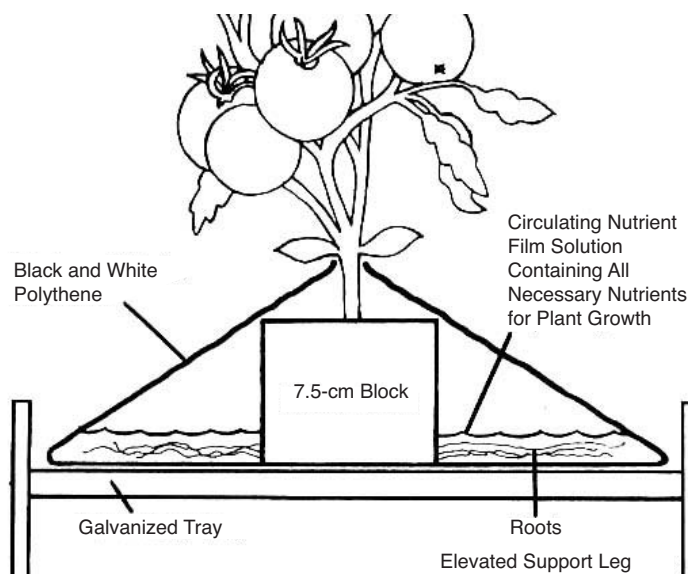
Figure 9.3 Cross-section of a NFT trough with a tomato plant rooted in a germination block with black/white polyethylene sheeting pulled up to and around the base stem of the plant to form a trough.
