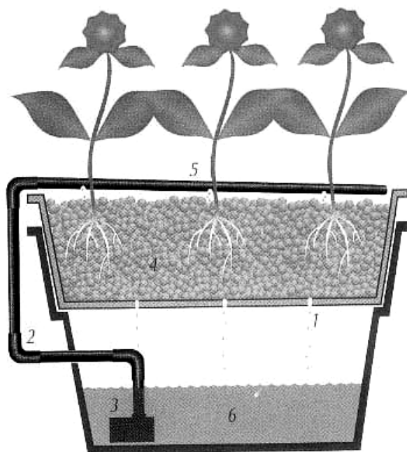
Figure 11.6 Drip system hydroponic growing vessel for growing vegetables (1: small holes in the base of the growing vessel allows applied nutrient solution to flow back into the nutrient solution reservoir (6), 2: nutrient solution delivery line, 3: pump, 5: drip irrigation line). Source: Coene, T., 1997, The Growing Edge 8(4):34–40.
