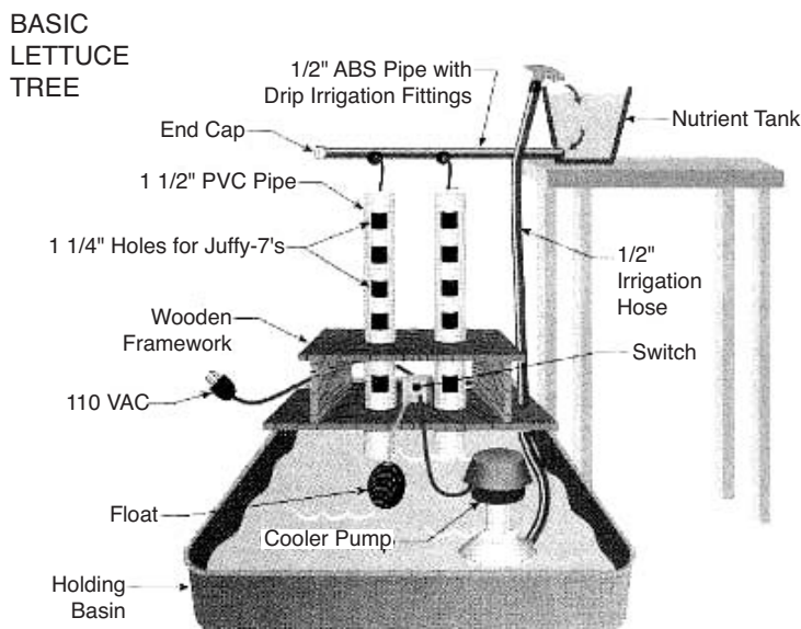
Figure 11.32–1 Design of the vertical NFT system developed by Cornell University for growing lettuce. Source: DeKorne, J.B., 1992–93. An orchard of lettuce trees: vertical NET system, The Growing Edge 4(2):52–55.
