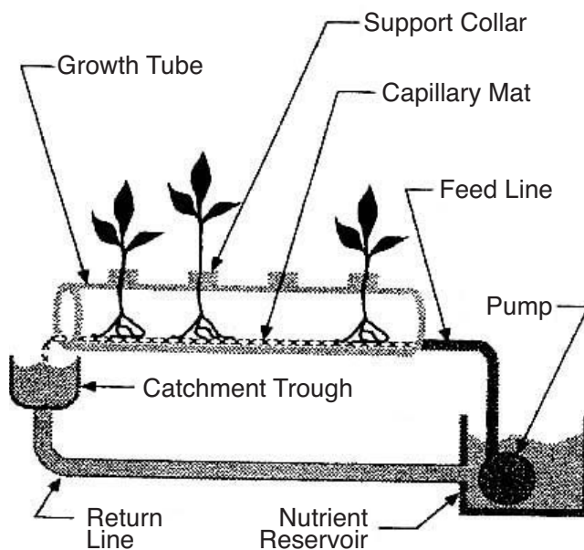
Figure 9.4 Typical arrangement for a home garden closed NFT system from which nutrient solution is pumped from a reservoir into a sloping growth tube with the nutrient solution flowing down the tube and back into the nutrient reservoir (Source: Van Patten, G.P., 1992, The Growing Edge 3(3): 24–33, 48–51).
