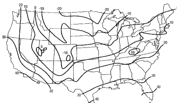
Figure 12.10 Winter design temperature map for estimating heat loss for the United States. Heat gain is indicated by the positive numbers for the year in the southern regions, and heat loss by negative numbers in the northern latitudes. Source: Bartok, J.W., Jr., 2000, Greenhouses for Homeowners and Gardeners, Cooperative Extension NRAES-137, Natural Resource, Agriculture, and Engineering Service (NRAES), Ithaca, NY.
