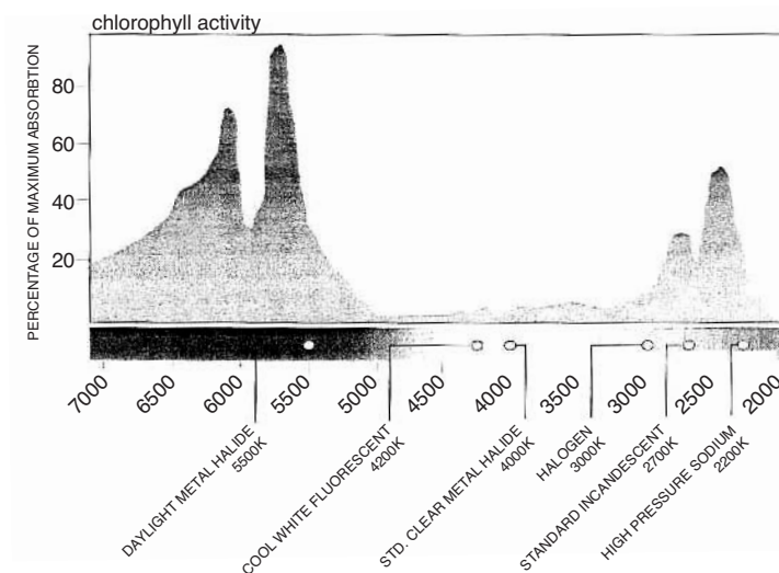
Figure 12.18–2. Chlorophyll activity as a percent of maximum absorption for various light sources. Source: Roberto, K., 2001, How-To Hydroponics , 3rd ed., Futuregarden, Inc., Farmingdale, NY.
