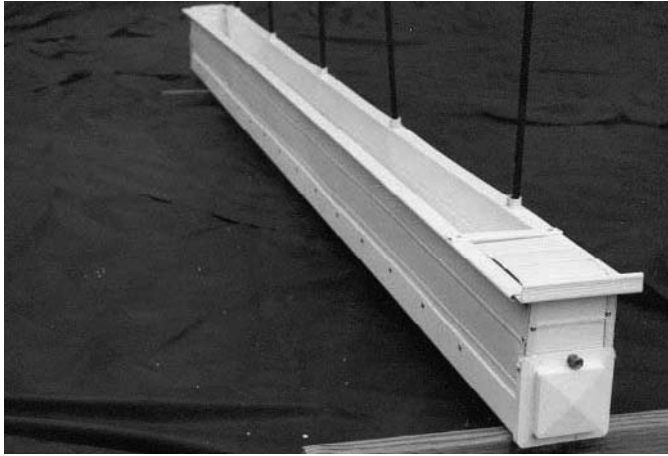
Figure 11.10–1 GroSystem GroTrough hydroponic system. (The lid on the front end of the trough covers the chamber that houses the float valve which is used to continuously maintain about a 1-in. depth of nutrient solution in the bottom of the GroTrough. The PVC side tubes are used to support the side walls of the trough and can be used to mount plant support stakes.)
