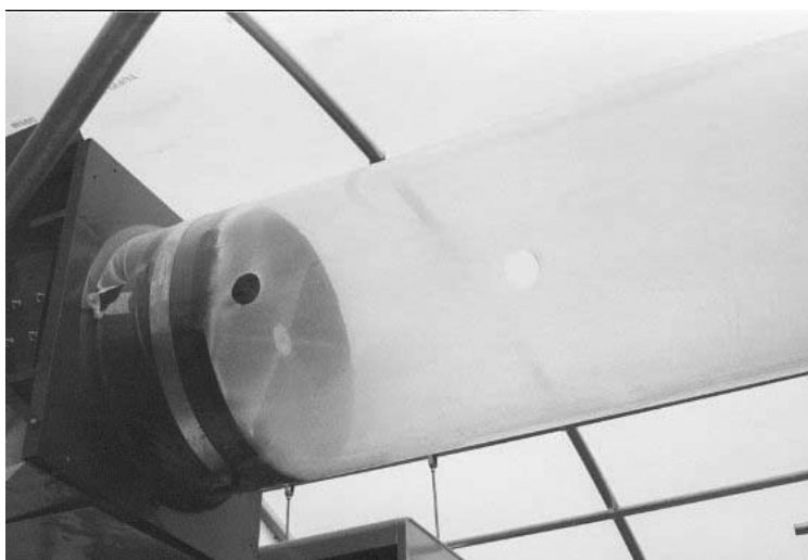
Figure 12.9 Fan-driven (see the fan in Figure 12.8) heated air is delivered through a large plastic-holed tube that runs the entire length of the greenhouse in the gable.
