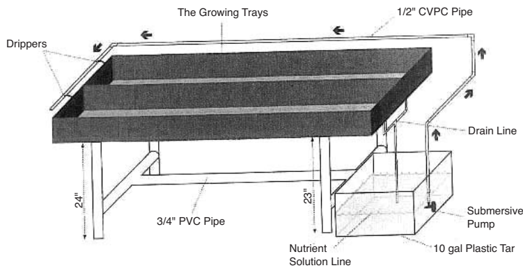
Figure 11.7 Drip system hydroponic growing tray for growing vegetables. Source: Creaser, G., 1997, The Growing Edge 8(3):68–73.
