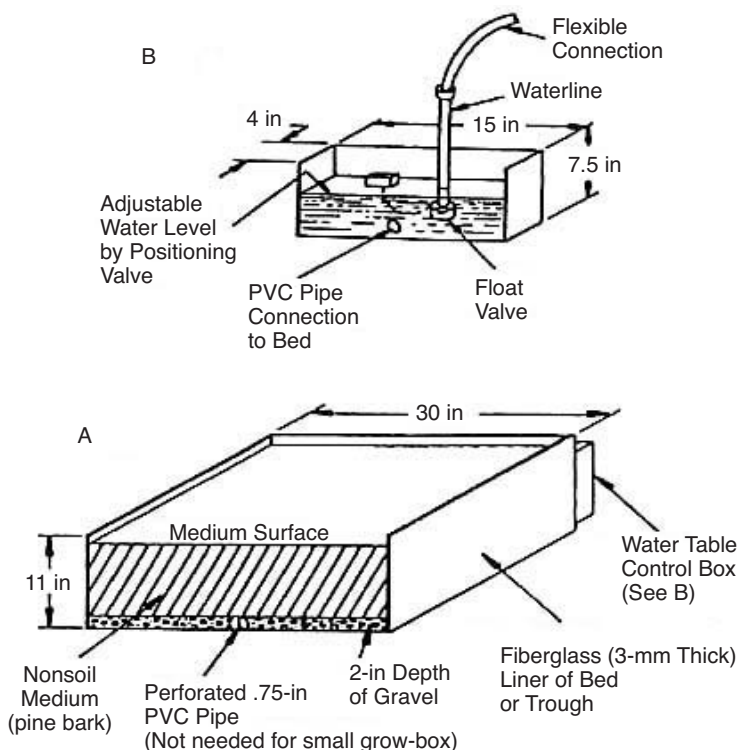
Figure 10.2 Pinebark grow-box system employing a constant water table with automatic water level control. Source: Jones, J.B., Jr., 1980. Construct your own automatic growing machine. Popular Science 216(3):87.
