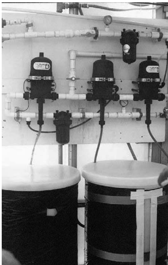
Figure 7.4–2 Dosers for dispensing stock nutrient solutions are shown in place over stock solution barrels. (Dosers are adjustable so that they can deliver a specific aliquot of stock nutrient solution into a flow of water for constituting a nutrient solution for delivery to plants. One doser is used for each stock nutrient solution.)
