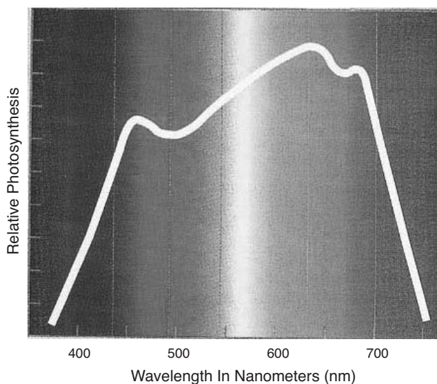
Figure 12.17 Relationship between wavelength and relative photosynthesis (Source: Parker, D., 1994a, The Growing Edge 5(4): 53–57, 66–67).
