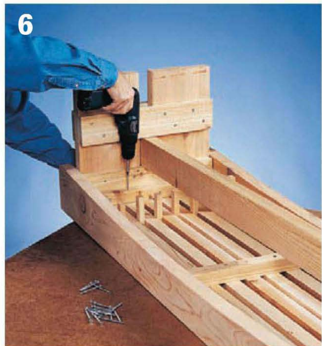
6 Attach the seat slats with glue and 2½" deck screws. Insert ½"-thick spacers to set gaps between the slats.
