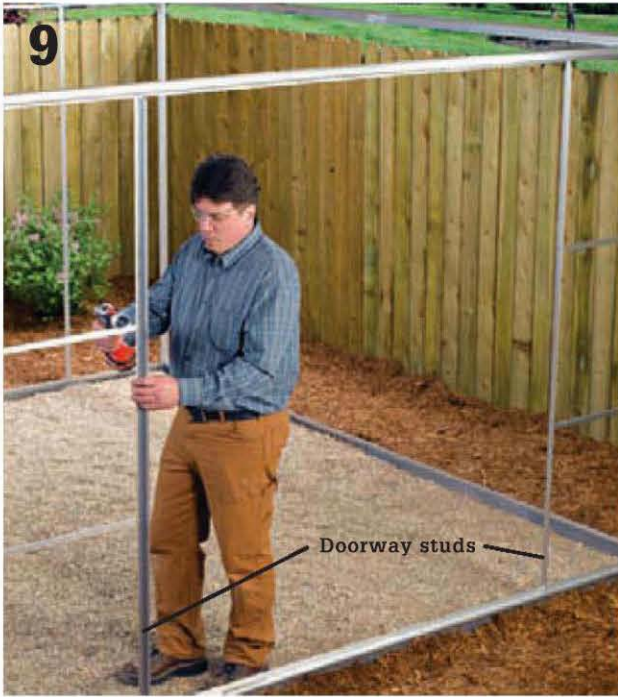
9 Install the doorway studs at either side of the greenhouse door, on the front end of the building. Install the side studs along both side walls of the greenhouse.
