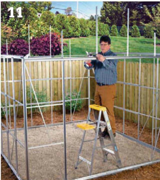
11 Fasten the gable-end stud extensions to the front and back walls of the greenhouse. The top ends of the studs should angle upward, toward the peak of the greenhouse.
