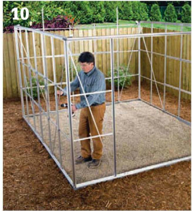
10 Add diagonal struts , as directed by the manufacturer. The struts help to stiffen and square up the walls. As you work, take diagonal measurements between opposing corners at the top of the walls, to make sure the structure remains square.
