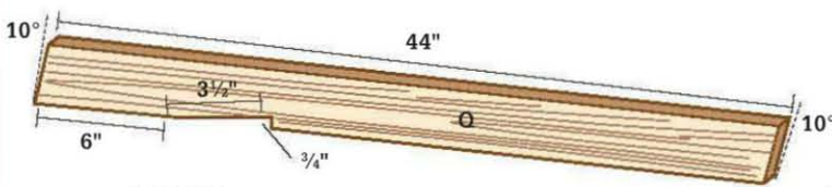
RAFTER
