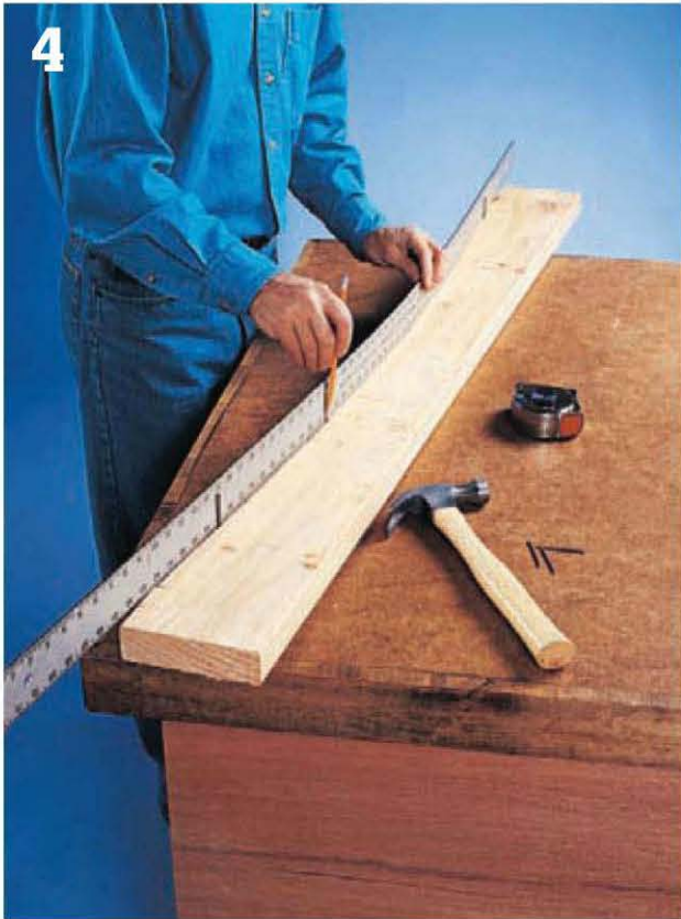
4 Mark the profile cuts on the aprons. Use a flexible ruler pinned between casing nails to trace a smooth arc.
