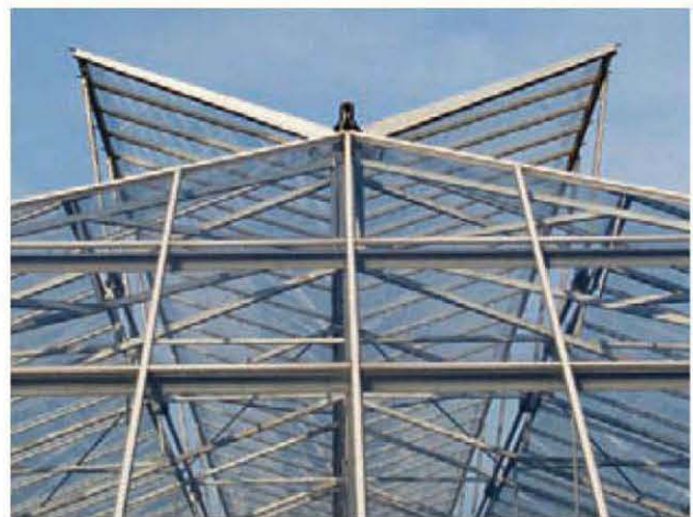
Roof vents that are triggered to open automatically by sensor alerts are far and away the most important component of a greenhouse cooling system. But additional cooling devices may be necessary.
