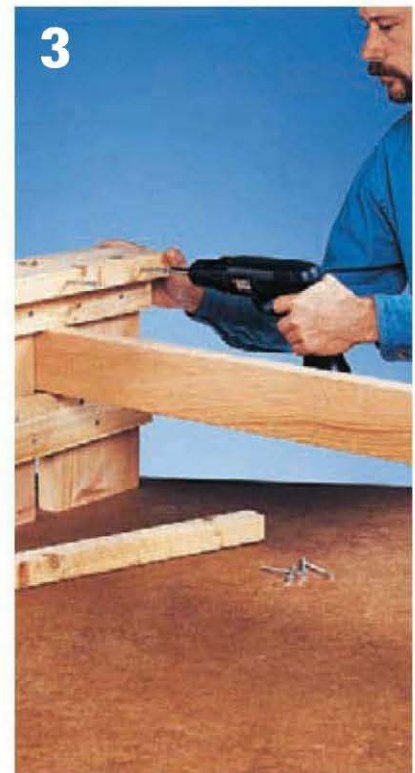
3 Attach the outer brace for the seat slats directly to the inside faces of the cleats.
