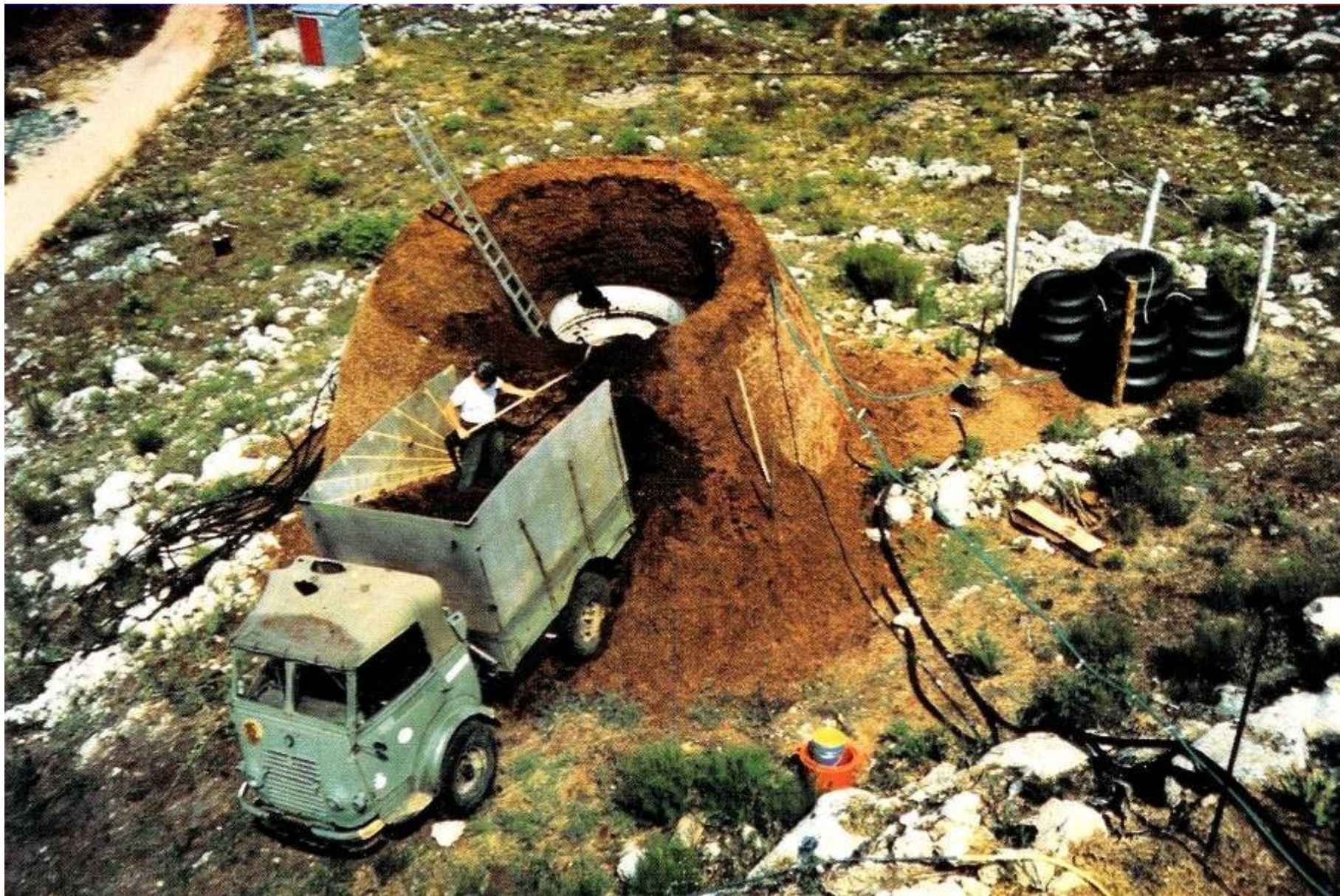
Loading the Brushwood Gas production tank by hand. (loading and emptying now done by automatic pump of our design.)
