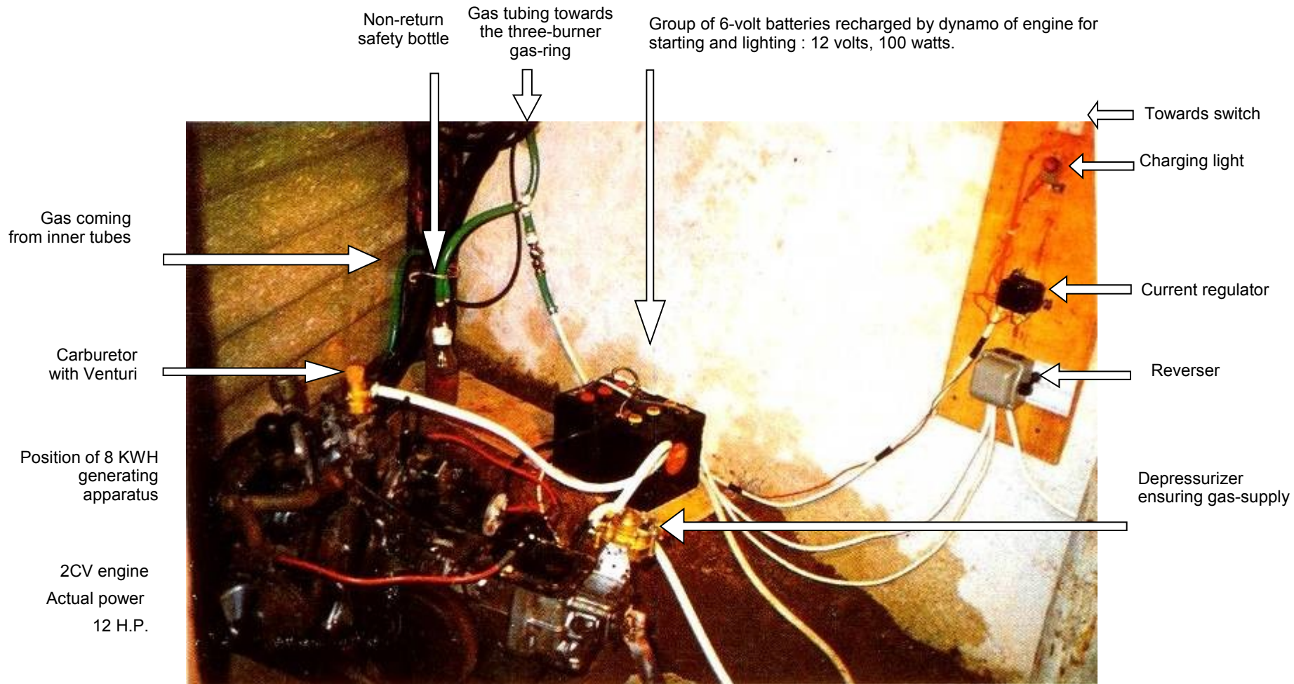
JANUARY 1979. – FIRST BRUSHWOOD GAS ELECTICITY PLANT. POTENTIAL POWER 8 KWH.
