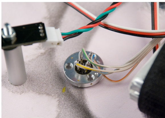
Figure 2-20. Wires soldered to RGB LED
