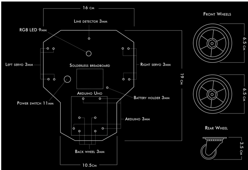
Figure 1-1. Blueprint of the chassis
