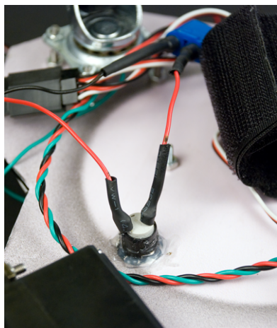
Figure 2-15. Positive wires soldered to the power switch
