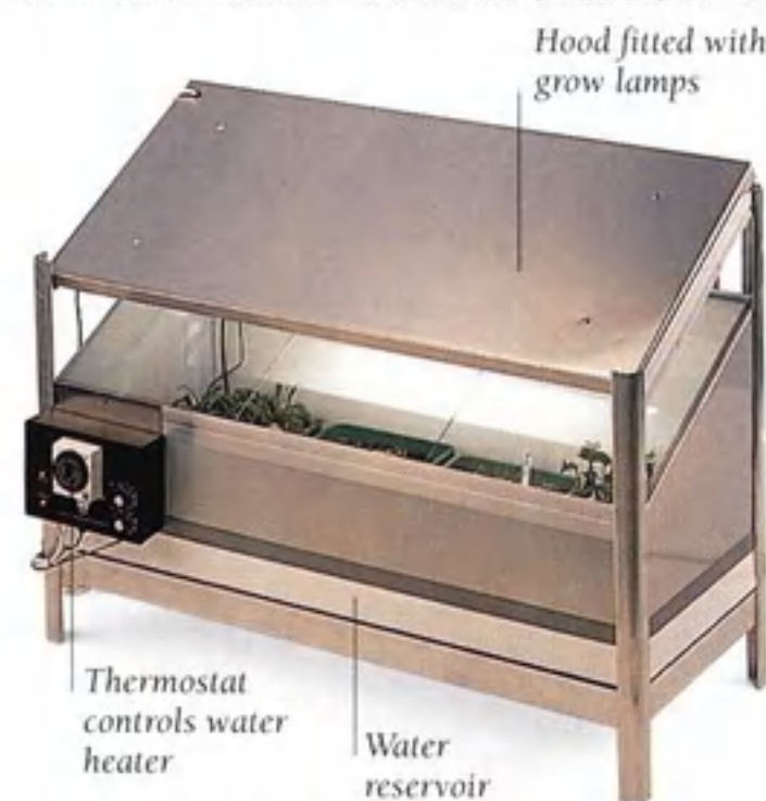
FOG PROPAGATION UNIT This unit pumps fresh air through a water reservoir, creating a warm "fog" around the propagated material without wetting the leaves. Vapor condenses on the sides and runs back into the reservoir.
